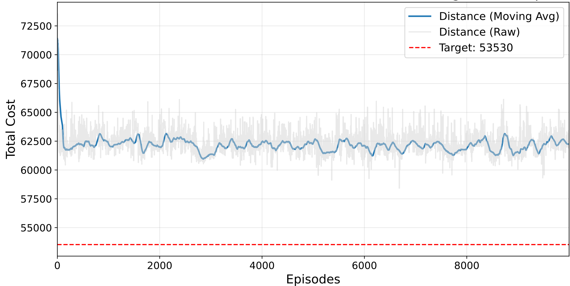
Final GAUSSIAN PROCESS Masked AutoRL-SOP Training - ft70.4.sop
